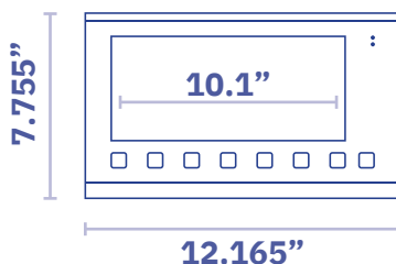
V500 Monitor Dimensions
