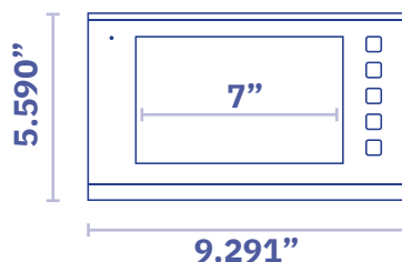
V500 Monitor Dimensions
